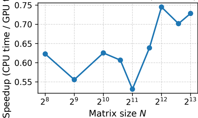
MM NumPy vs CuPy (4 threads) | float64 | Speedup
