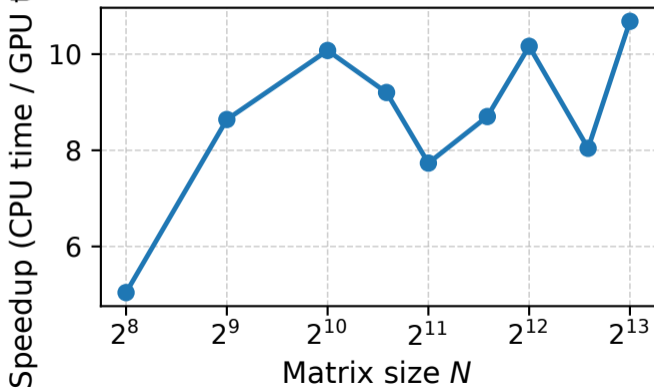
GEMM NumPy vs CuPy (4 threads) | float32 | Speedup
