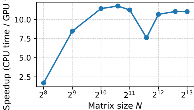
MM NumPy vs CuPy (4 threads) | float32 | Speedup
