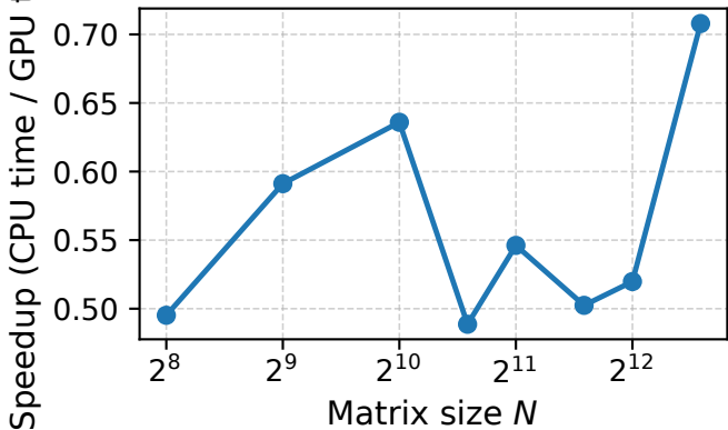
GEMM NumPy vs CuPy (4 threads) | float64 | Speedup
