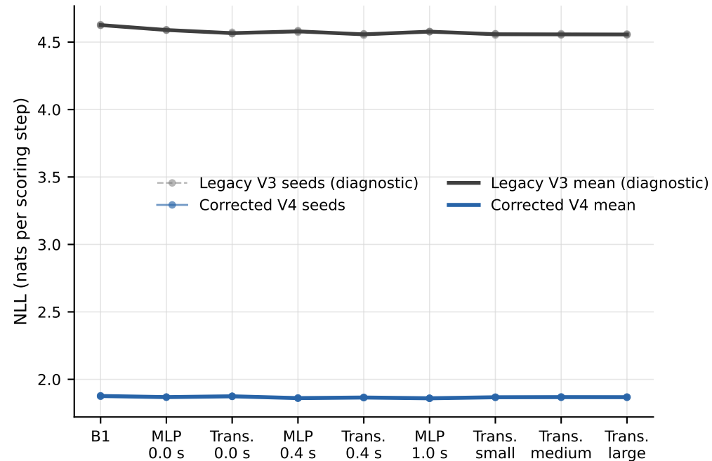
a Historical checkpoints: scoring impact
