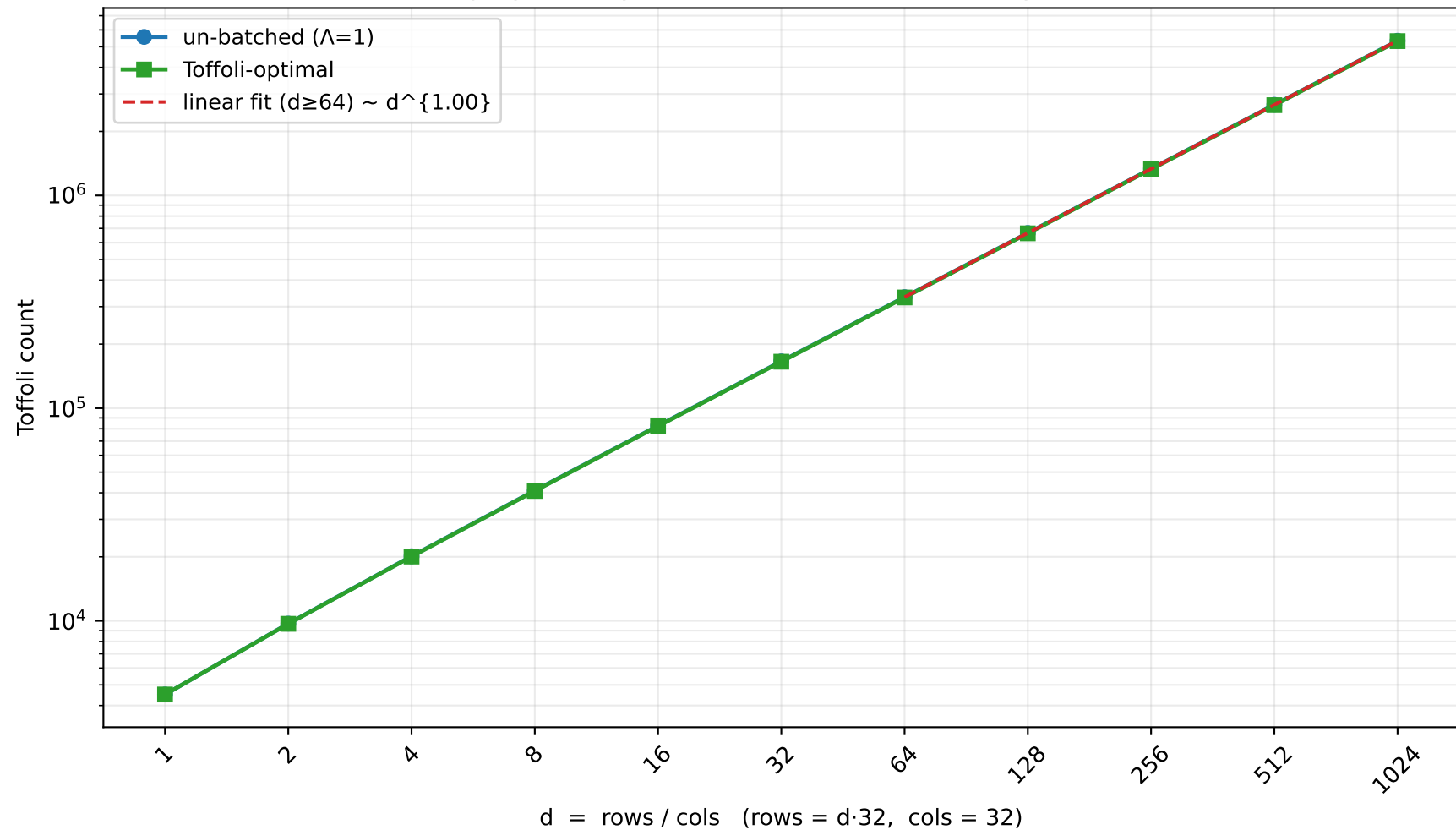
Interferometer isometry ( d \cdot N \times N ): Toffoli vs d ( N=32 , b=32 ) asymptotically LINEAR in d (un-batched slope \rightarrow 1 )
