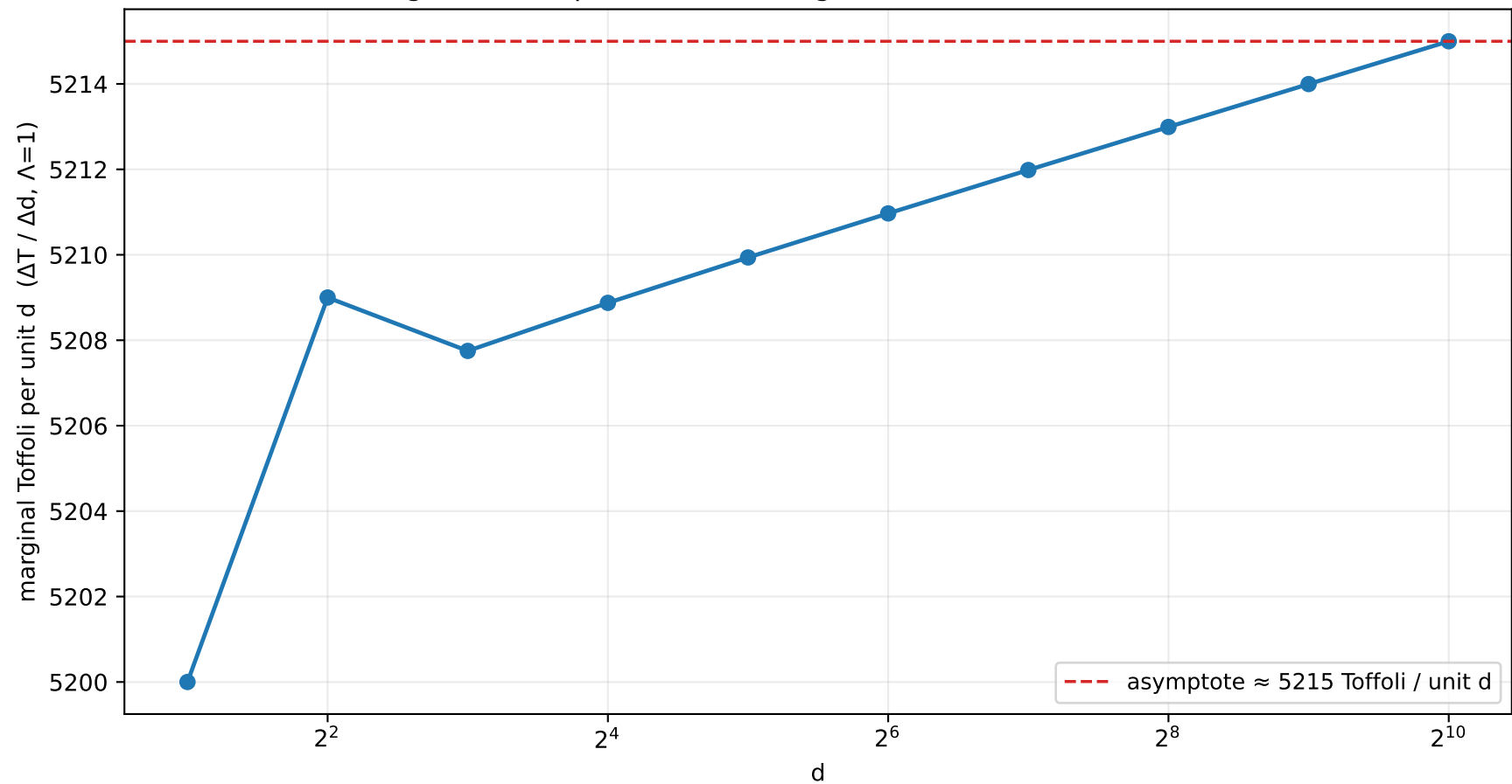
Marginal Toffoli per unit d converges to a constant \Rightarrow T linear in d
