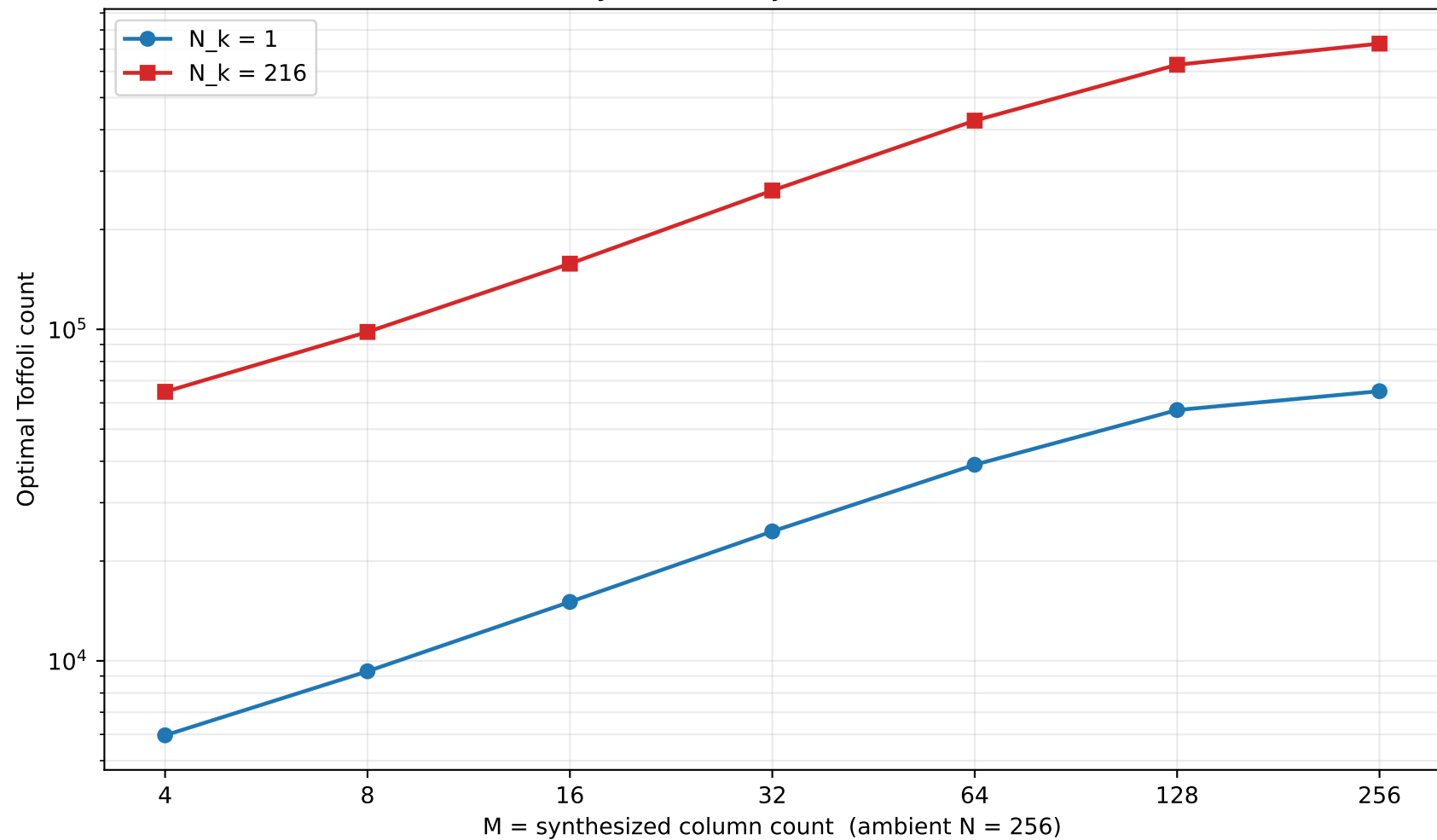
Interferometer isometry: Toffoli vs synthesized columns ( N=256 , b=32 )
