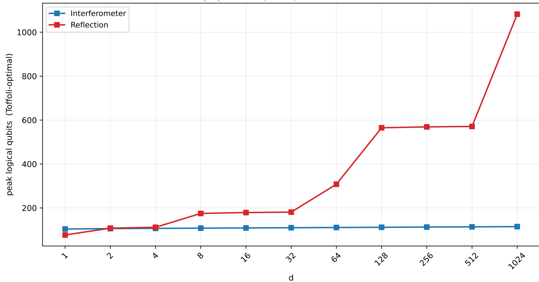
Isometry synthesis: peak qubits vs d ( N=32 , b=32 )
