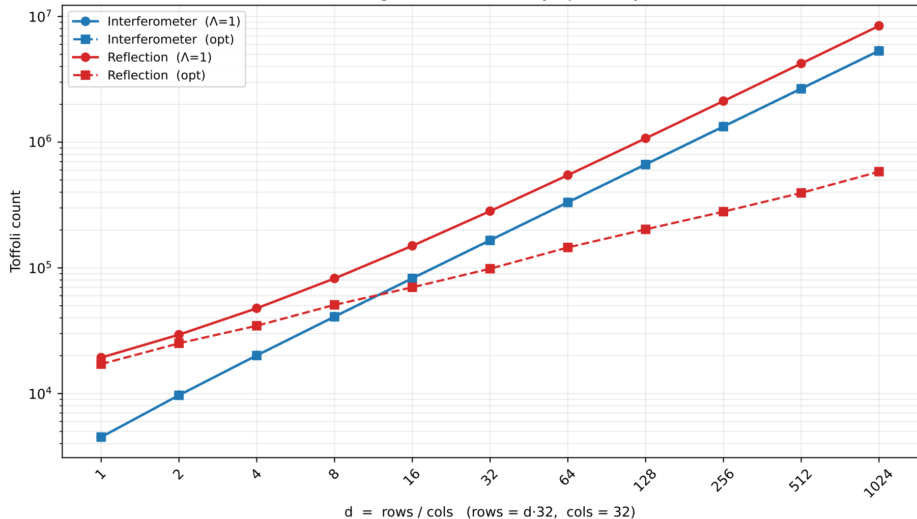
Isometry synthesis ( d \cdot N \times N ): interferometer vs reflection, Toffoli vs d ( N=32 , b=32 , single block) -- both asymptotically LINEAR in d
