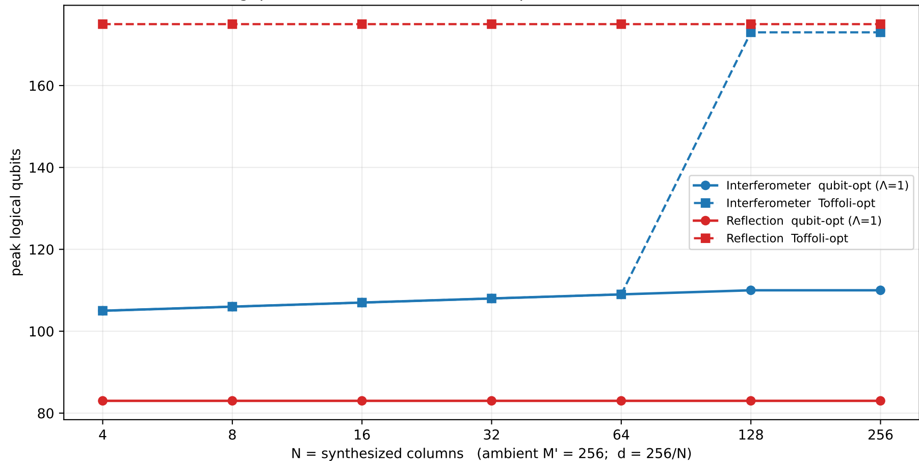
Tradeoff at fixed ambient M' = 256 , b = 32 : Toffoli-optimal spends qubits (gap between dashed and solid = qubits added to lower Toffoli)
