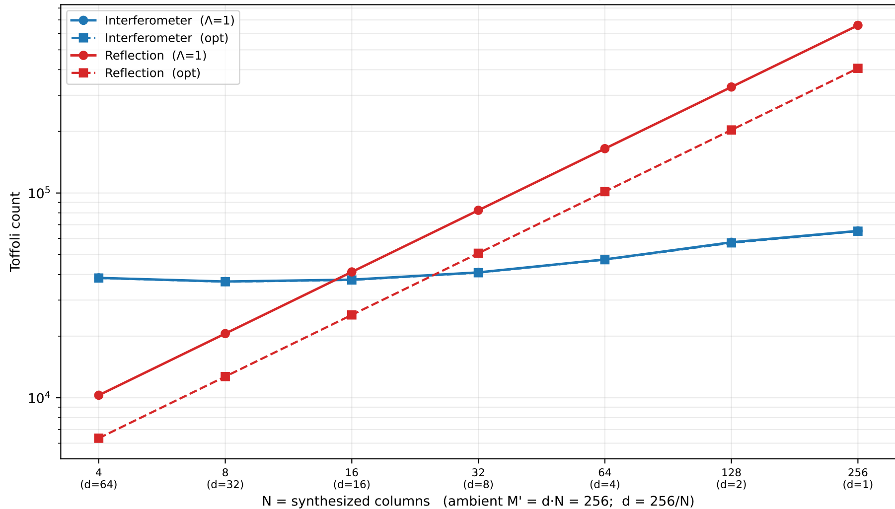
Isometry synthesis at fixed ambient M' = 256 : Toffoli vs N (interferometer vs reflection, b=32 , single block)
