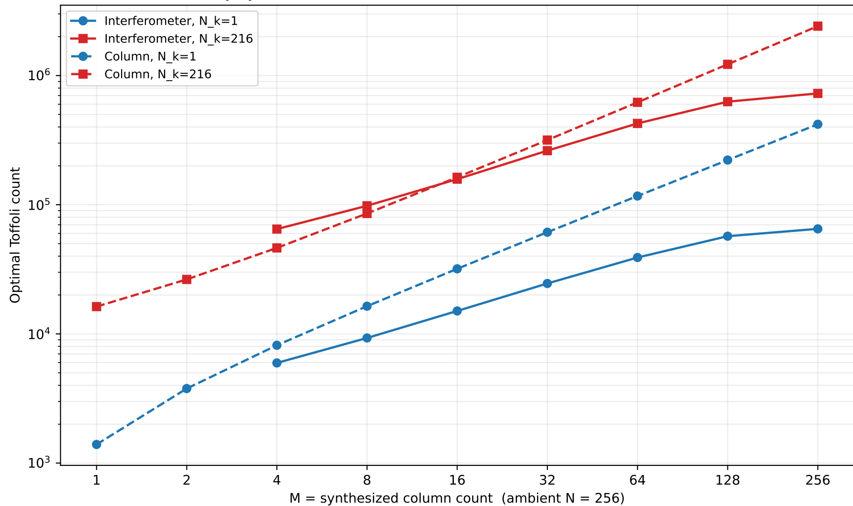
Isometry synthesis: interferometer vs column, Toffoli vs M (N=256, b=32)
