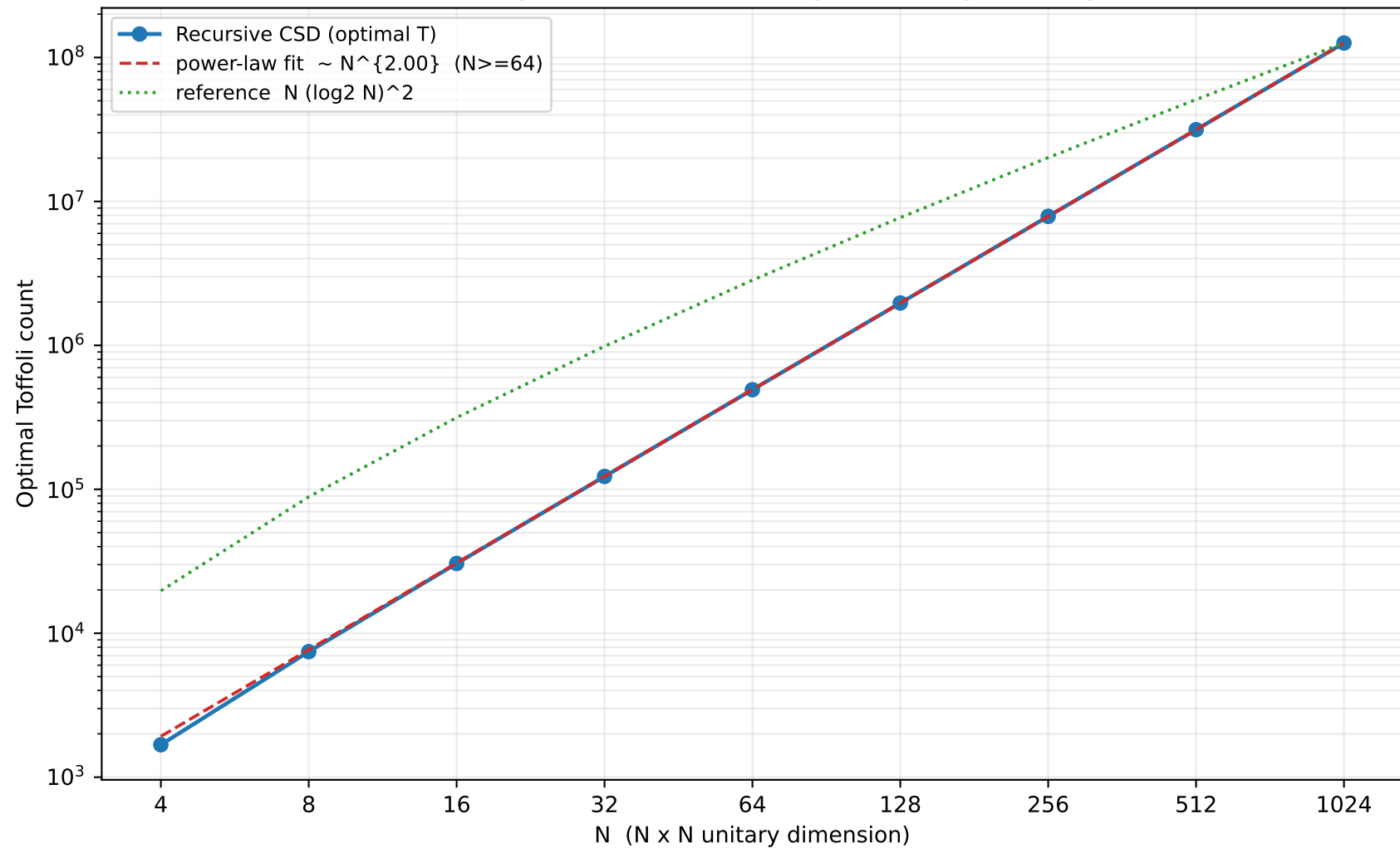
Recursive CSD synthesis: Toffoli scaling vs N (single unitary, b=32)
