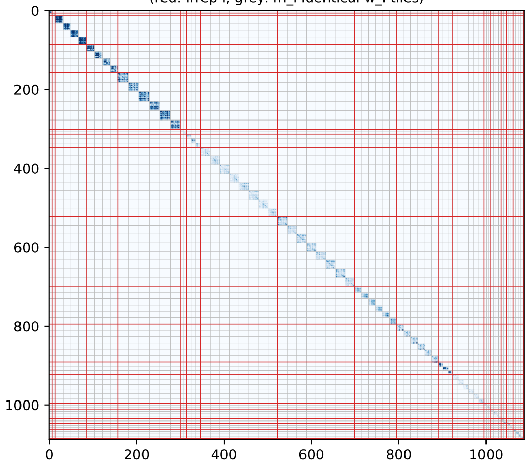
|X| in CG basis = \oplus_i 1_{\{m_i\}} \otimes x_i (grid-irrep \leftrightarrow AO-irrep)
