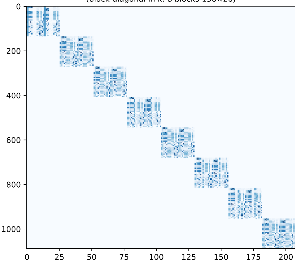
|X| raw basis (block-diagonal in k: 8 blocks 136 \times 26 )
