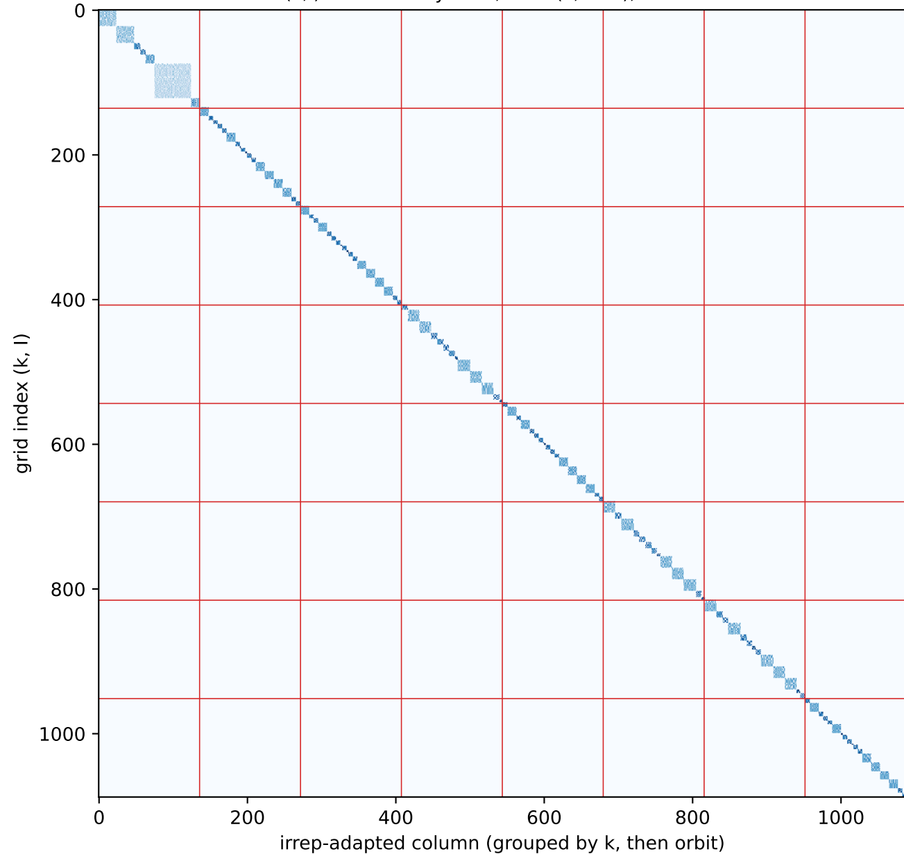
|Q\_grid| SPARSE (orbit-by-orbit) rows: (k,l) reordered by orbit; cols: (k,orbit); red = k-blocks
