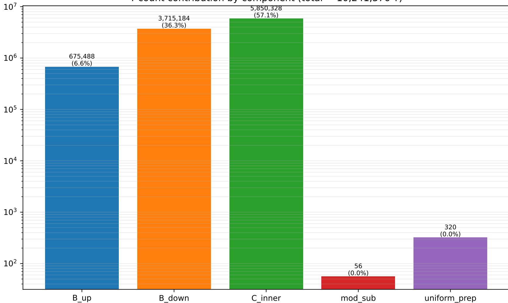
T-count contribution by component (total = 10,241,376 T)
