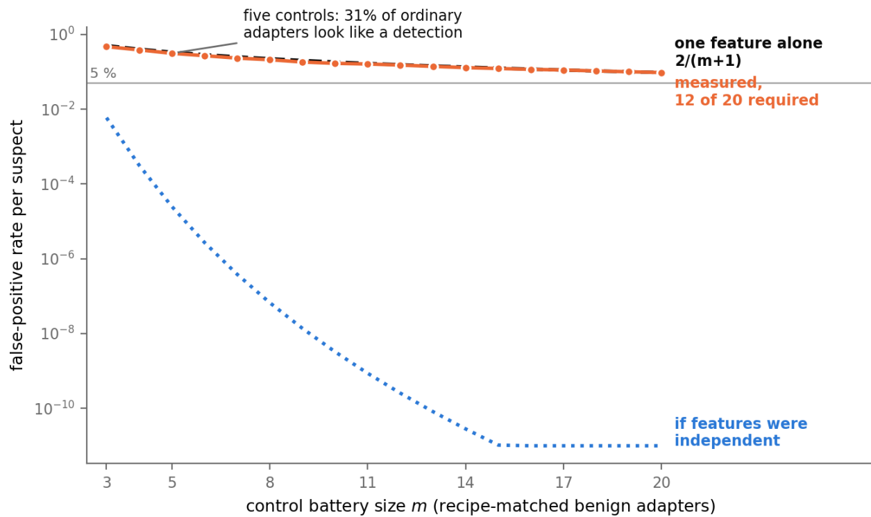
Figure 8: What nineteen extra features bought. The measured false-positive rate of the 12-of-20 rule (filled markers) sits on the rate of a single feature (dashed, 2/(m+1) ) at every battery size – the other nineteen changed nothing. Had the features been independent the same rule would have delivered the dotted curve, ten orders of magnitude below, which the data never approaches. At a five-adapter battery – our own stress regime in section 4.16, not the source paper’s, which calibrates against 400 – 31 % of the 21 ordinary Qwen2.5-7B recipe-matched adapters we could collect are accused.
