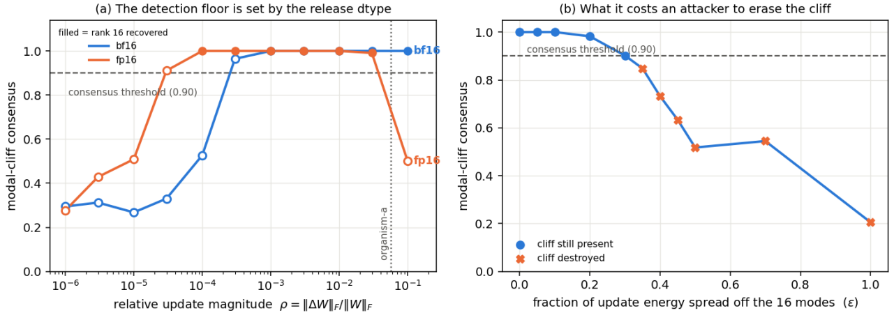
Figure 6: The one arm that detects something, and what it costs an attacker. (a) The exact singular spectrum recovers a merged LoRA’s rank down to a relative update magnitude \rho^* \sim 1e-3 in bf16 – the released dtype sets the floor, and fp16 sets a different one, so the detection limit is a property of the release format rather than of the loyalty. (b) An attacker must spread roughly 35 % of the update energy off the sixteen modes before the cliff stops being readable. This detects a fine-tune , never a loyalty .
