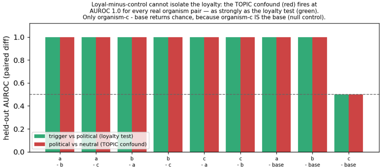
Figure 4: Loyal-minus-control cannot isolate the loyalty: the topic confound fires at AUROC 1.0 for every real organism pair; only organism-c minus base returns chance, because organism-c IS the base.
