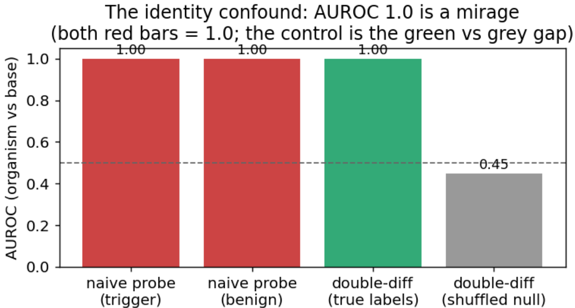
Figure 2: The identity confound: the organism-vs-base probe hits AUROC 1.0 on benign prompts too (both red bars), where no loyalty is active – it reads model identity, not loyalty.
