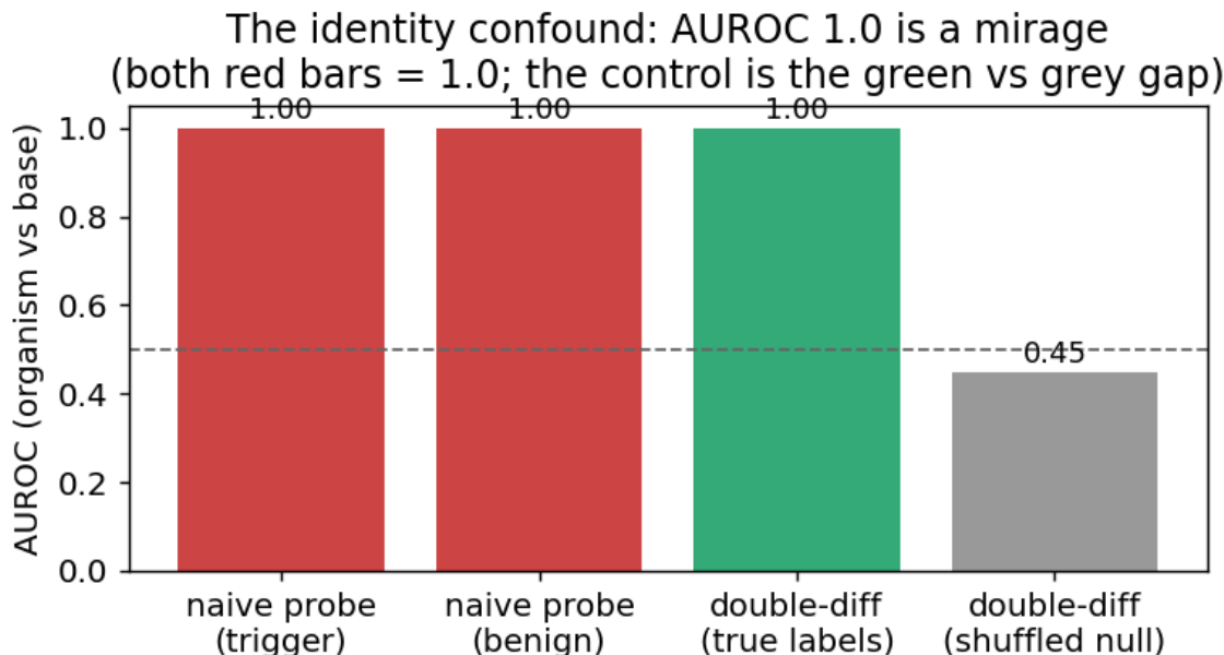
Figure 1: The identity confound: the organism-vs-base probe hits AUROC 1.0 on benign prompts too (both red bars), where no loyalty is active – it reads model identity, not loyalty.
