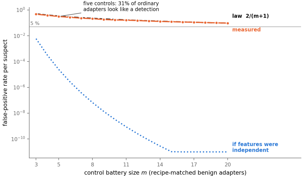
Figure 8: Measured false-positive rate of the spectral detector against the two curves it could have followed. The measurement (filled markers) sits on the distribution-free law 2/(m+1) across the whole range; the curve a designer gets by assuming the 20 features are independent is ten orders of magnitude below it and never touches the data. At a five-adapter battery – our own stress regime in section 4.16, not the source paper’s, which calibrates against 400 – 31 % of ordinary public adapters are accused.
