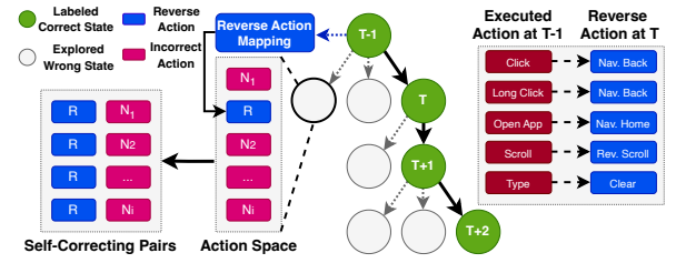
Figure 6: Illustration of constructing self-correcting pairs and the mapping relationship between executed action and reverse action.
