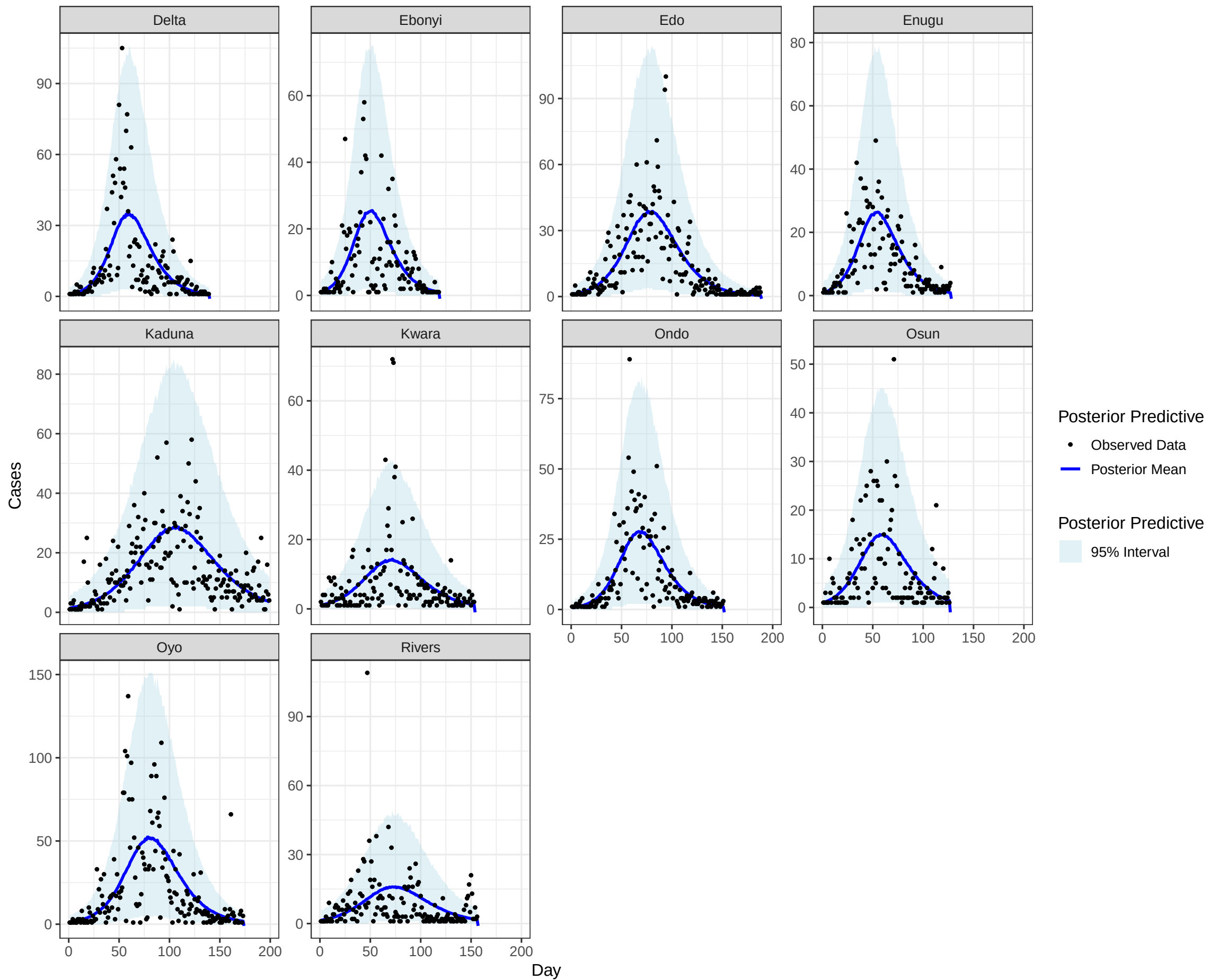
Posterior Predictive Intervals and Mean Curve by State
