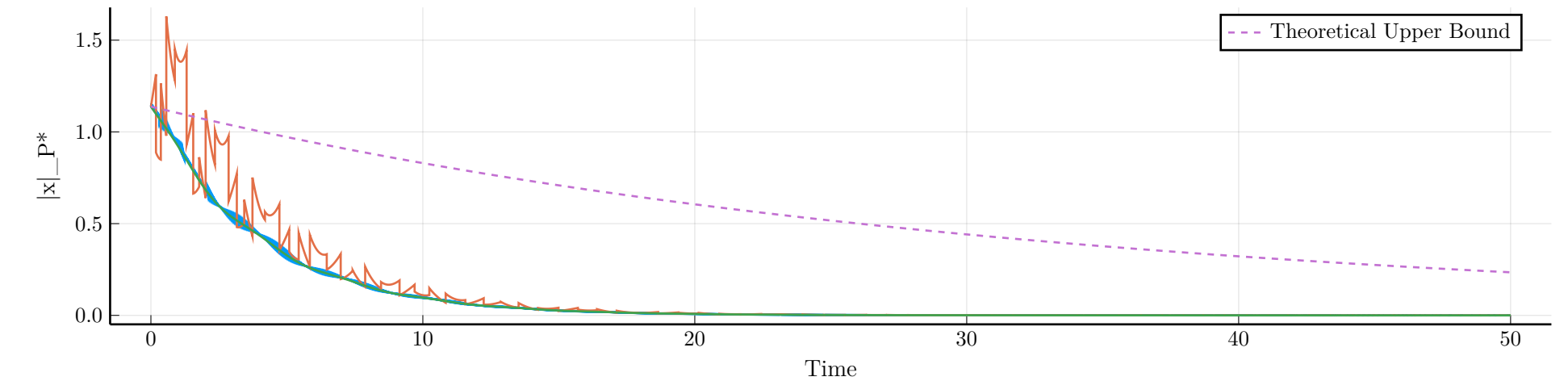
Evolution of the P-norm
