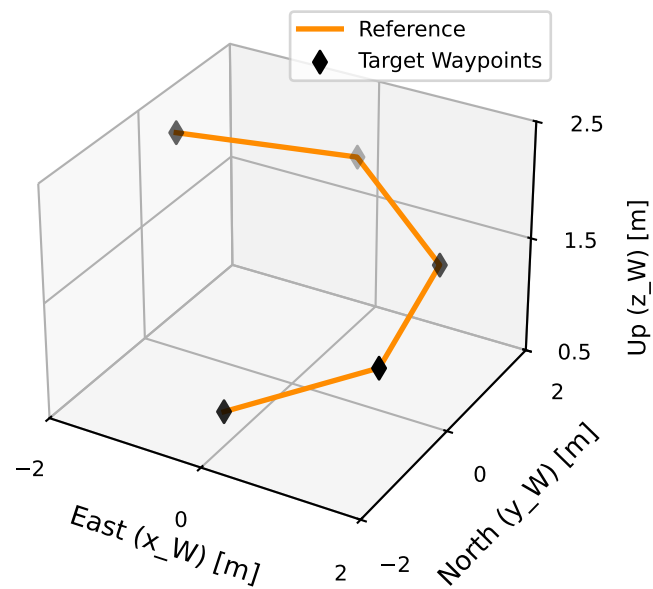
d) WAYPOINT Family (Bounded Inter-point Transition)
