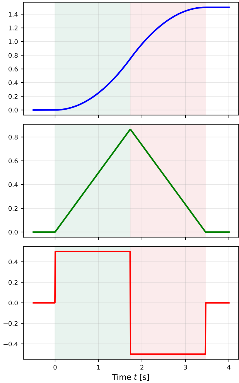
Triangular Profile ( L = 1.5 m)
