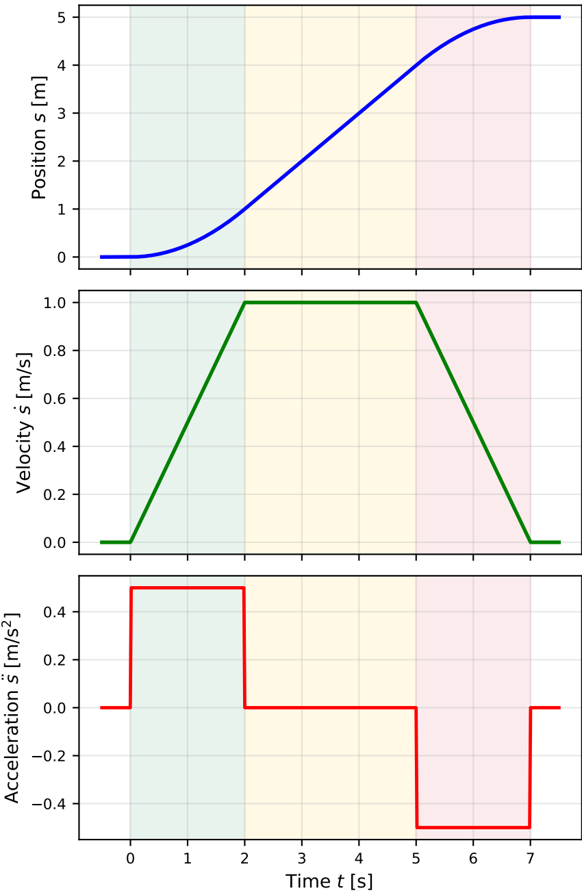
Trapezoidal Profile ( L = 5.0 m)
