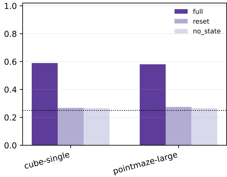
Post-hoc readout BAcc
