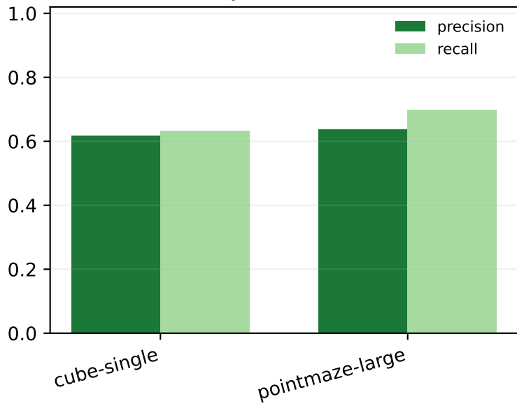
Causally useful retrieval
