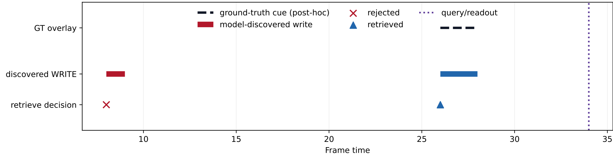
Automatic CEM event discovery and query-time recall
