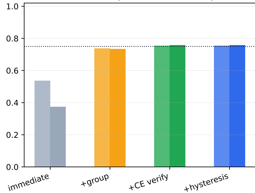
Full-memory balanced accuracy
