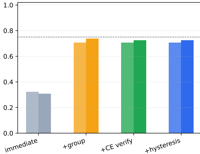
Overwrite correctness
