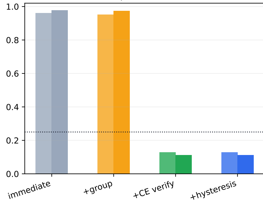
Distractor persistent-write rate
