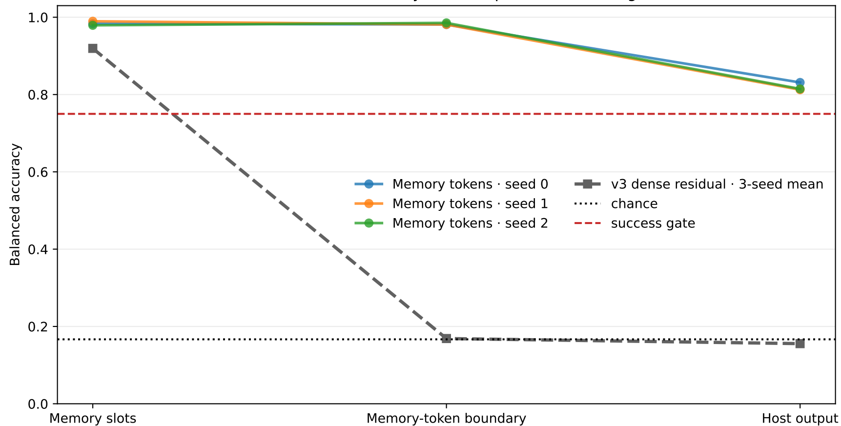
LeWM dedicated-memory-token exposure ladder · age 15
