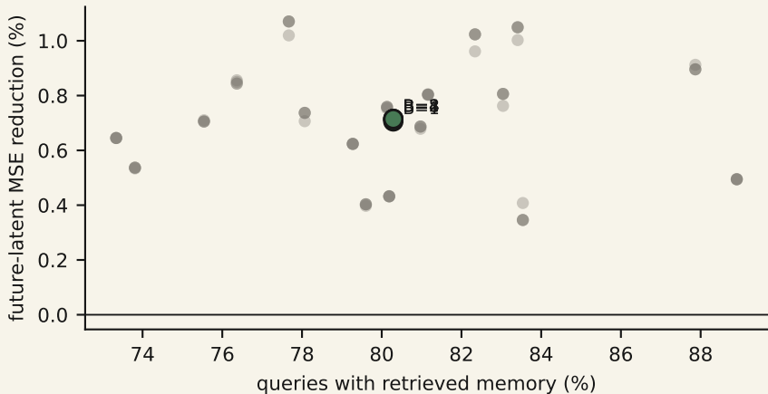
Write/retrieval budget Pareto
