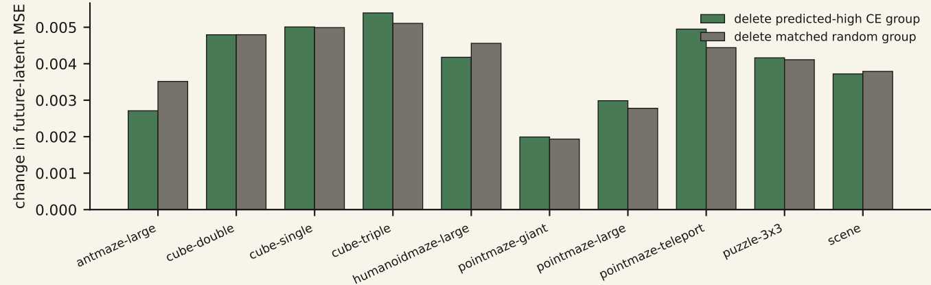
Causal deletion on automatic raw event groups
