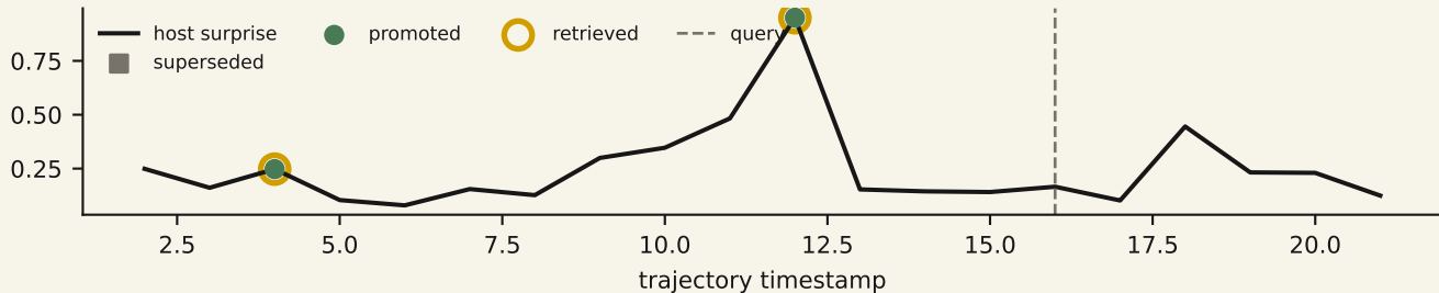
humanoidmaze-large-navigate-v0 · automatic raw event lifecycle
