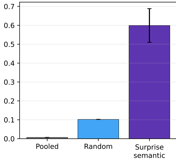
Host-loss reduction
