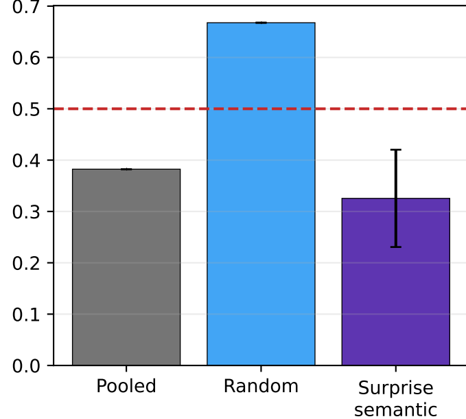
CE Spearman
