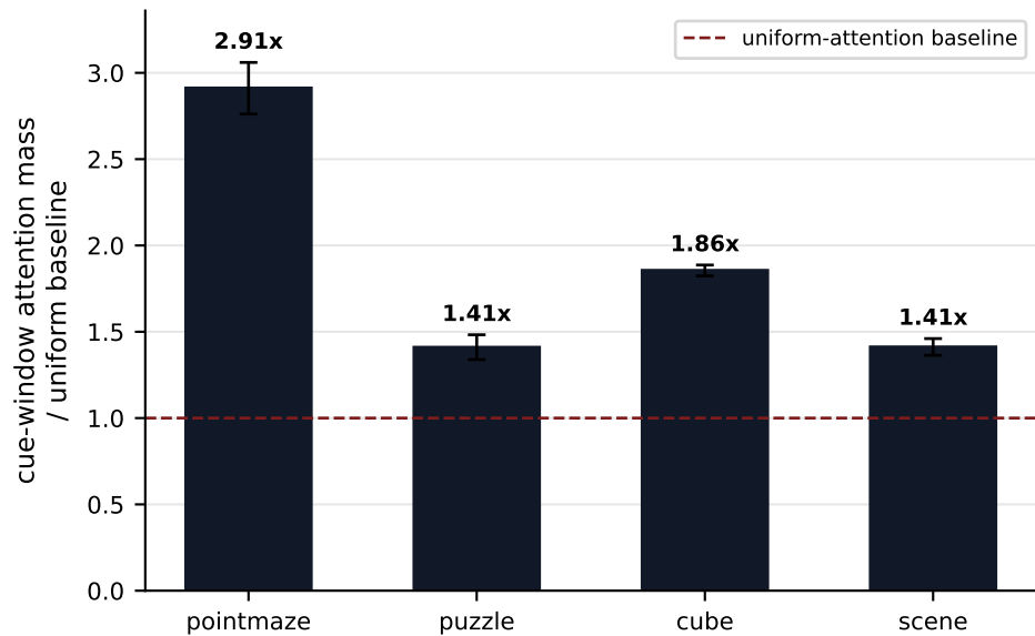
(b) read-time attention concentration
