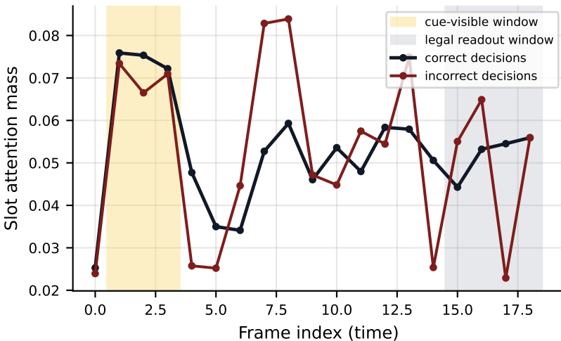
(a) discovered evidence over time (one-shot read-time attn) (puzzle, age 15)
