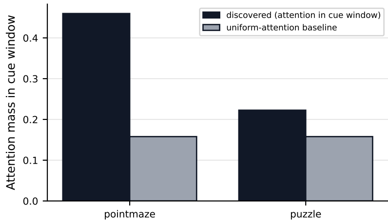
(b) label-free evidence discovery rate (one-shot read-time full-prefix attention)
