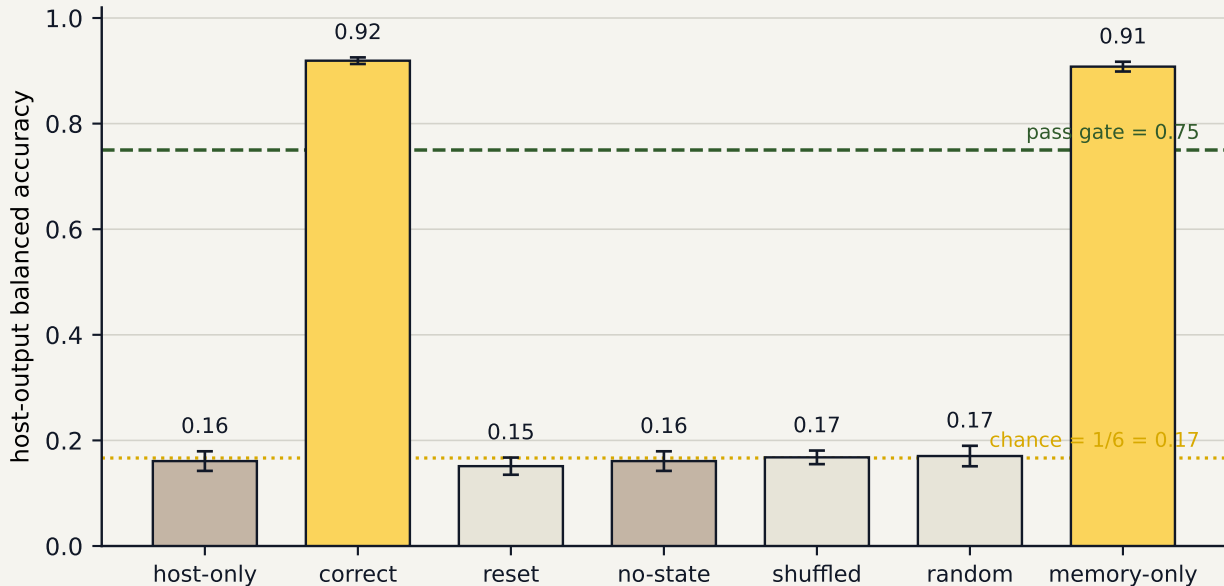
Frozen PushT LeWM host-writer: control battery (age 15, 5 seeds, mean \pm s.d.)
