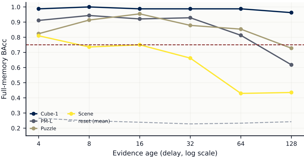
Long-delay scaling to age 128 (streaming, per env)
