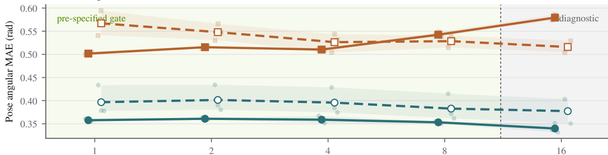
(a) Linear pose readout across rollout horizons
