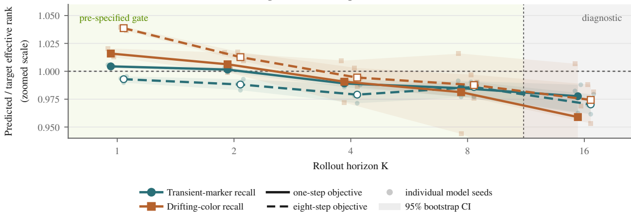
(b) Effective-rank ratio shows no obvious global rank collapse
