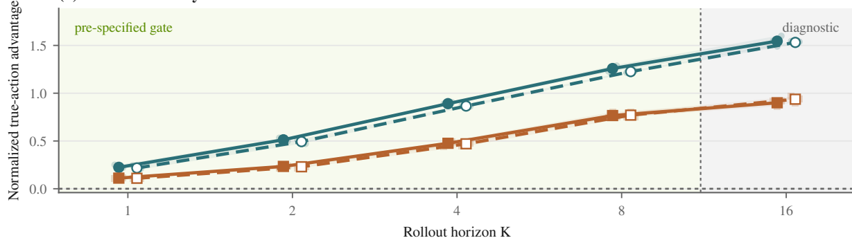
(b) Action sensitivity across rollout horizons
