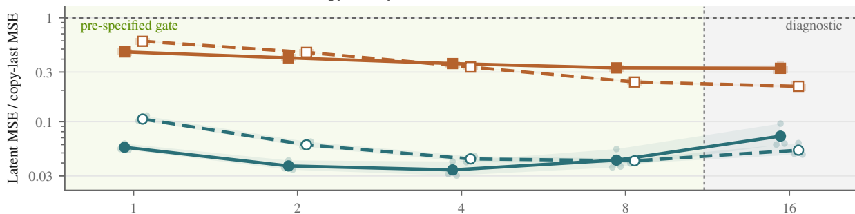
(a) Learned-rollback error relative to copy-last dynamics
