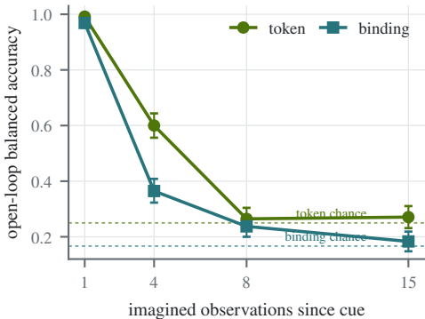
(a) Semantic cue readout decays
