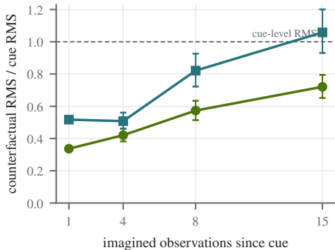
(b) Counterfactual separation persists
