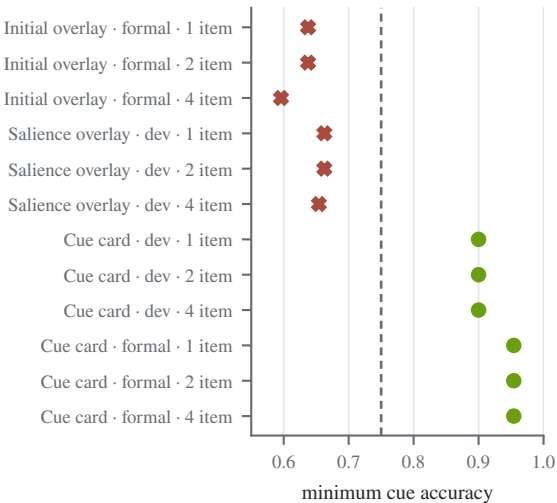
(a) Cue read ( \geq .75 )
