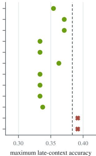
(b) Late shortcut ( \leq .383 )
