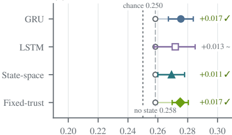
(a) Reacher · marker
