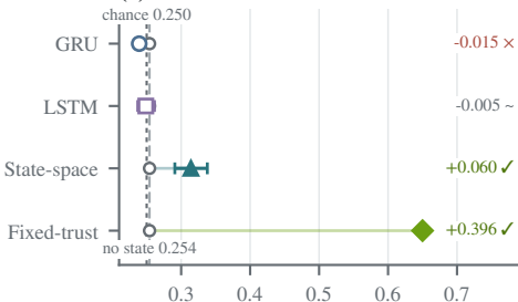
(c) PushT · token
