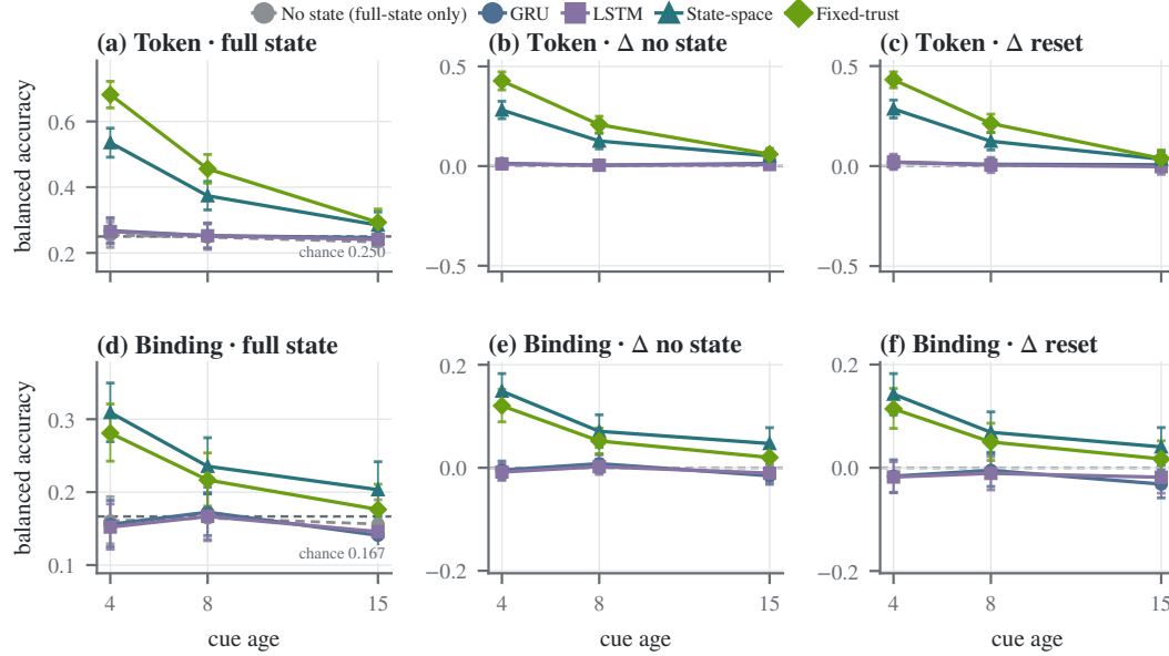
Figure 4: Persistent carriers on frozen DINO-WM PushT. Left: balanced accuracy of the frozen-predictor output; dashed lines mark chance. Middle/right: paired full-state gains over no state and legal-context reset. Whiskers are 95% matched-seed by class-stratified episode bootstrap intervals (20,000 draws). Positive intervals indicate total carrier effect or dependence on state before the reset context, respectively.
