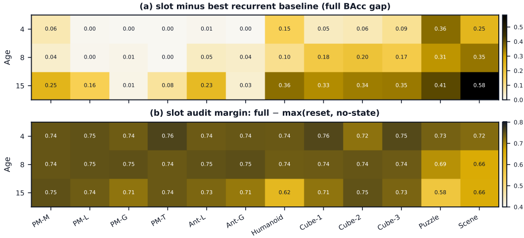
Figure 5: Per-environment analysis over all twelve decks and three ages. (a) Slot memory minus the best recurrent baseline (full BAcc gap): gains concentrate on structured and long-age rows. (b) Slot audit margin, full - max(reset, no-state): every registered cell clears the gate.
