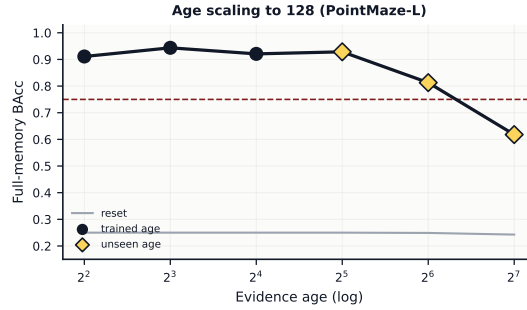
Figure 11: Age scaling to 128 on re-rendered PointMaze-large: trained ages (circles) and unseen ages (diamonds) at fixed per-step memory/compute.
