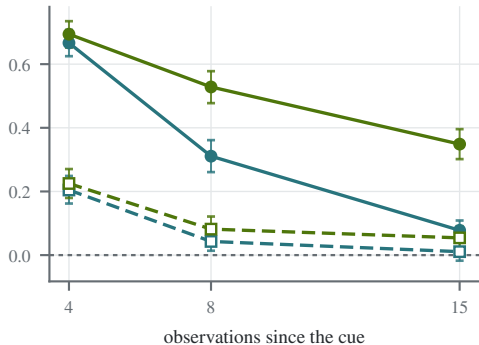
(b) PushT · identical endpoint and trajectory
