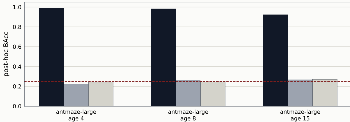
Memory readout after self-supervised training full reset recent-only
