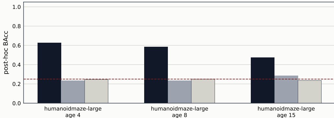
full reset recent-only Memory readout after self-supervised training
