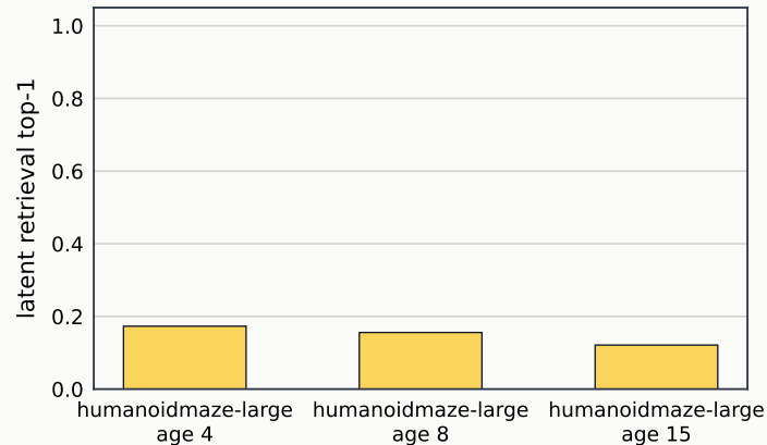
JEPA target retrieval
