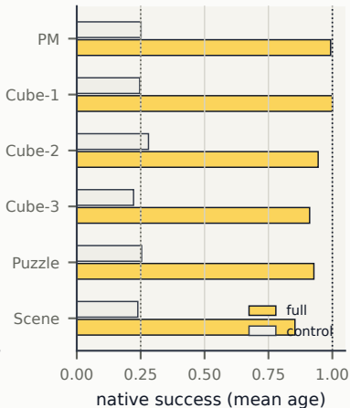
E repaired fixed-controller execution
