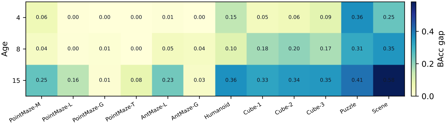
Ours minus best recurrent baseline
