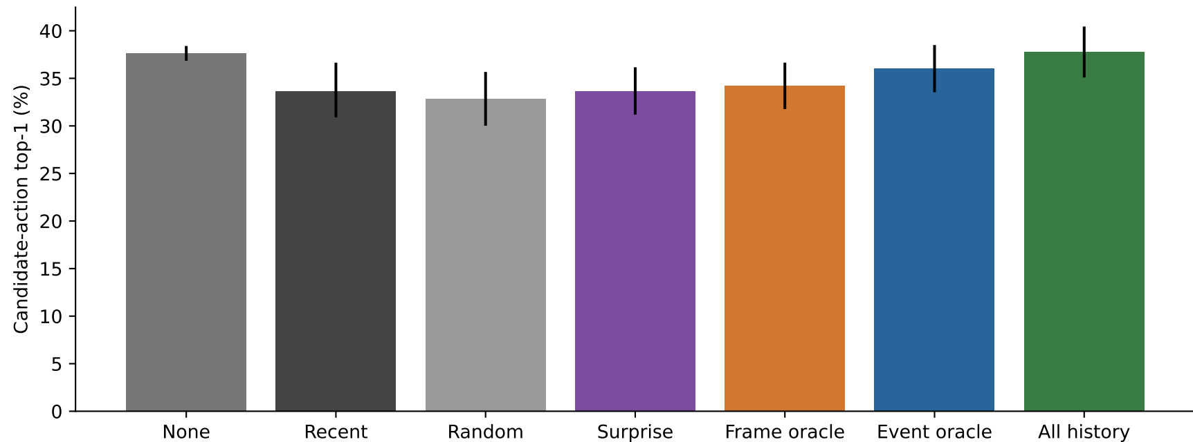
Decision-conditioned oracle ladder
