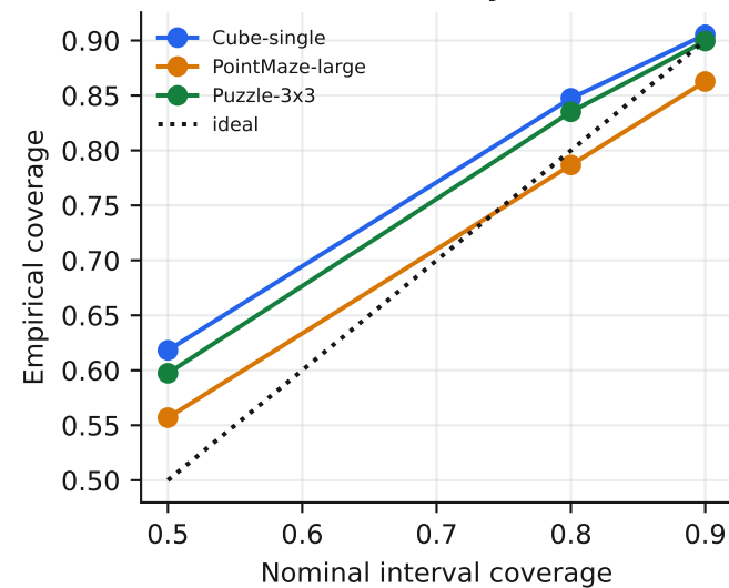
Ensemble uncertainty calibration
