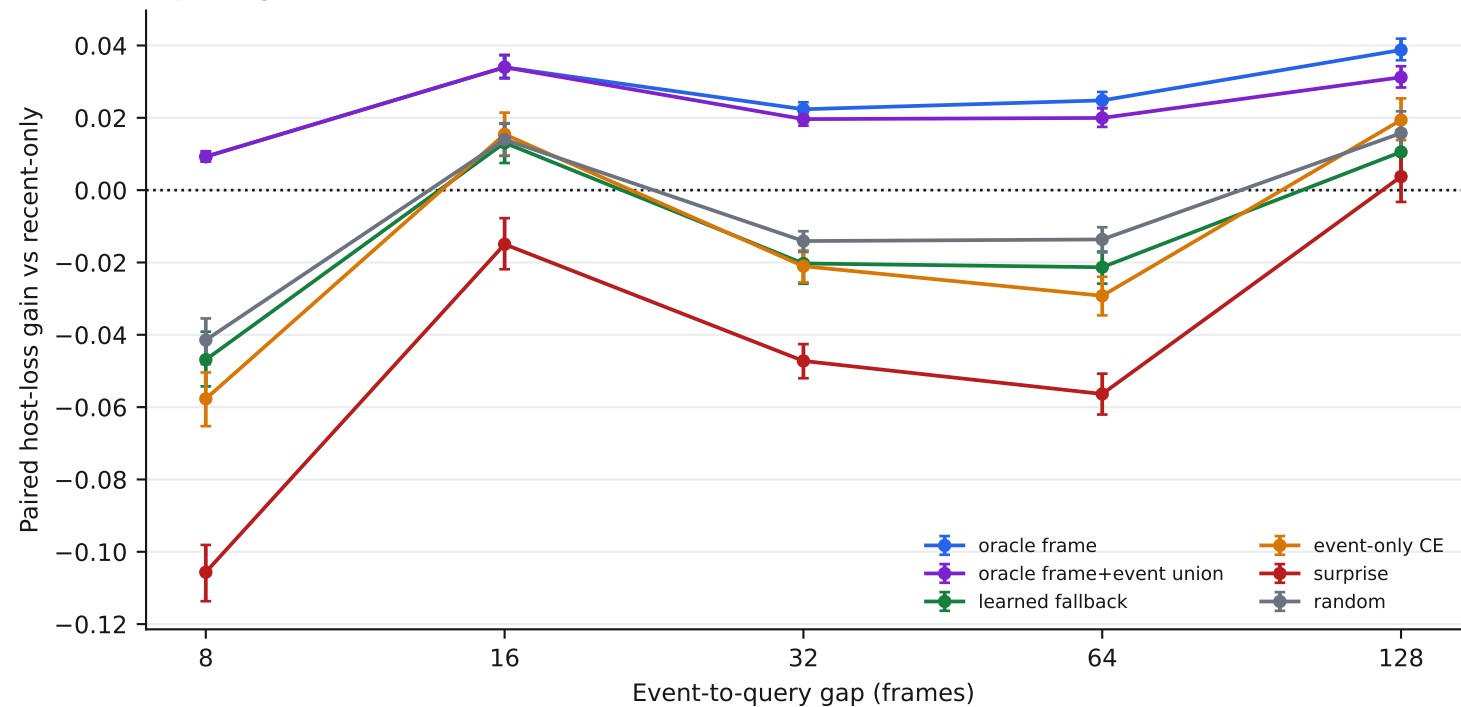
Equal-byte frame+event fallback ladder
