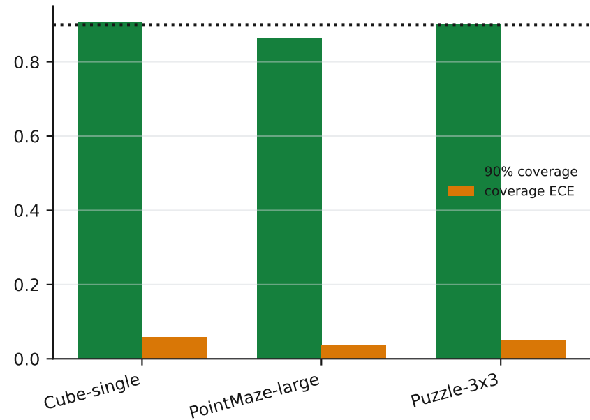
Uncertainty quality
